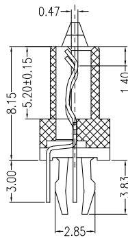
SECT C-C
