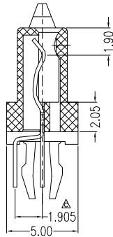
SECT B-B
