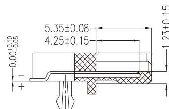
SECT B-B
