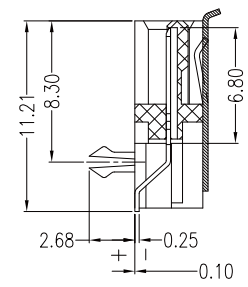
SECT B-B
