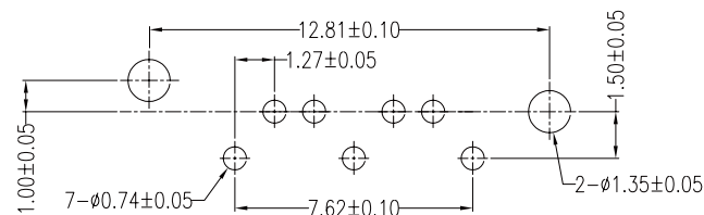
PCB LAYOUT
