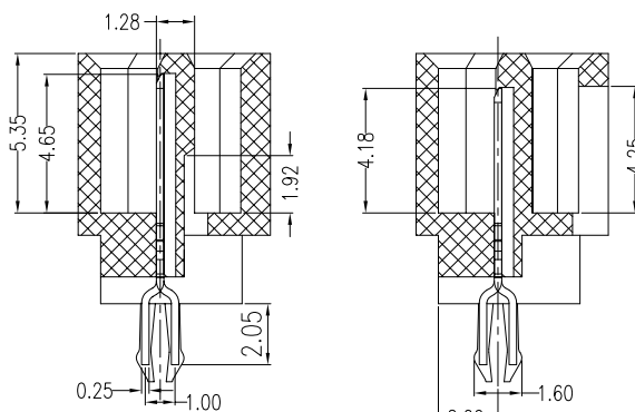
SECT B-B
