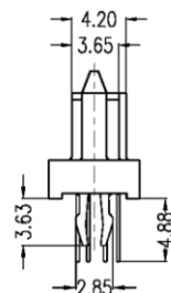
VIEW Q SCALE 2:1
