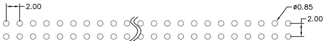
Recommended P.C.B Layout
