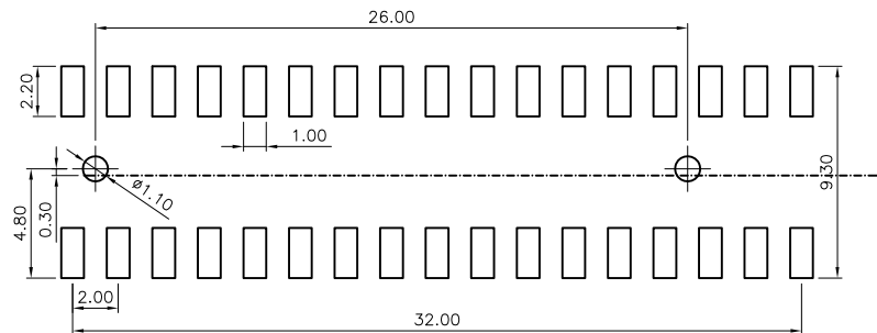
Recommended P.C.B.Layout
