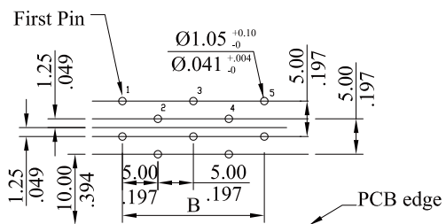
R Type PCB layout for normal
