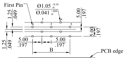
L Type PCB special layout for normal
