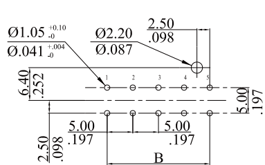
B Type PCB layout
