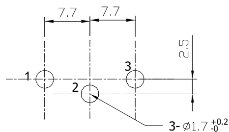
MOUNTING HOLE DETAILS
