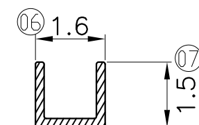
SEC C-C
