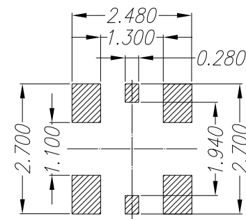
Recommend Stencil Mask Pattern (Mask Thickness 0.08mm)
