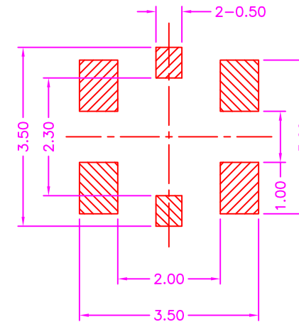
RECOMMENDED STENCIL MASK PATTERN
