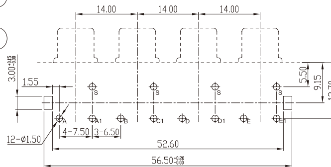
P.C.B LAYOUT TOL=0.1mm (BOTTOM VIEW)
