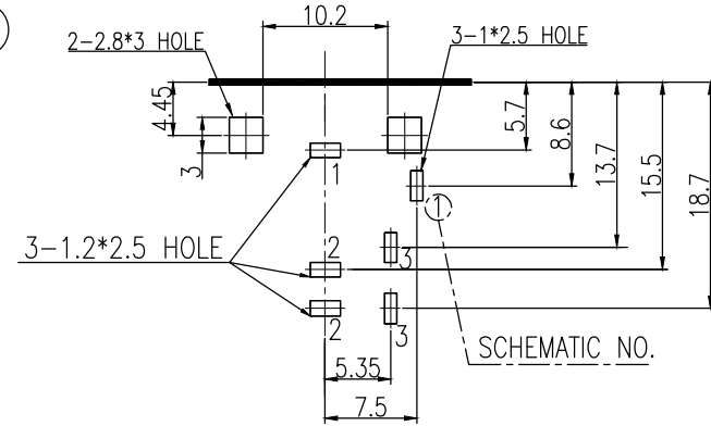
T:1.56 Dimensions of PC board holes Tolerance : ±0.1(Printed-BOTTOM view)
