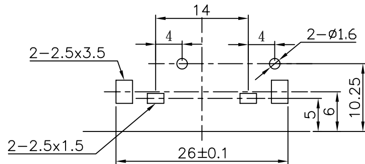
PCB HOLES ( TOP VIEWED )
