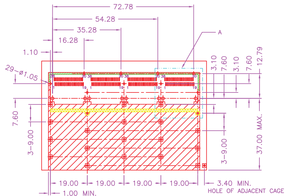
RECOMMENDED SINGLE SIDE PC BOARD LAYOUT
