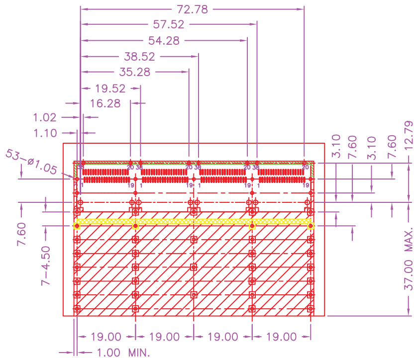
RECOMMENDED BELLY TO BELLY BOARD LAYOUT
