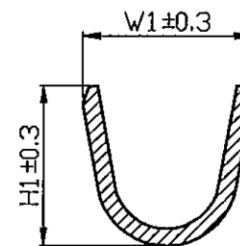
SECTION A-A S=10/1
