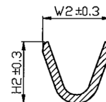
SECTION B-B S=10/1
