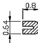
SECTION C-C S=10/1
