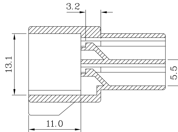
B-B SECTION
