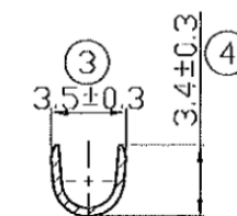
SEC. B-B
