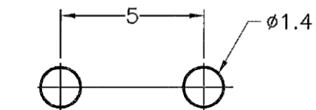
MOUNTING HOLES
