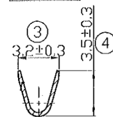
SEC. B-B
