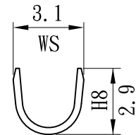
B-B Section
