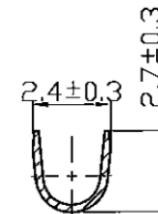
SEC. B-B
