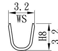
B-B Section
