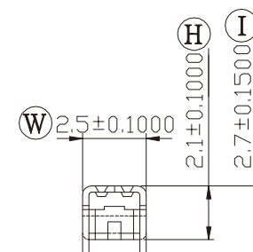
SEC.C-C
