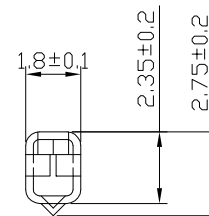
SEC.C-C
