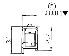
SEC. B-B
