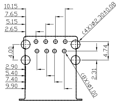
RECOMMENDED PCB DIMENSIONS -COMPONENT SIDE
