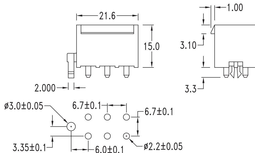
P. C. board hole dimensions
