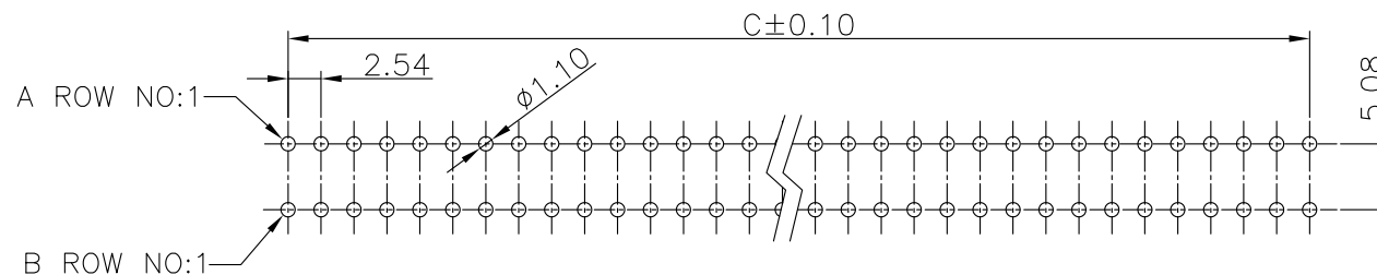
P.C. Board Layout (Tolerance: \pm 0.05 )
