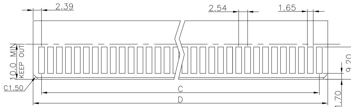
RECOMMENDED MATTING BOARD FOOTPRINT (Tolerance: \pm 0.05 )
