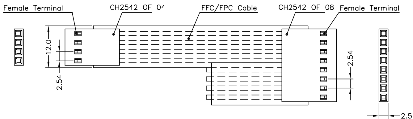
B Type: Female housing To Female housing
