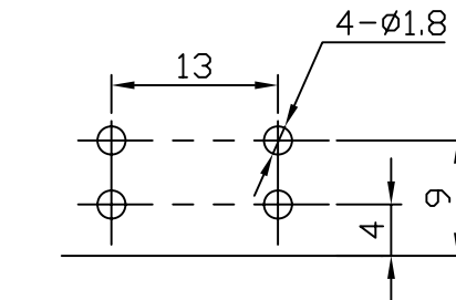
T:1.6 Dimensions of PC board holes Tolerance : ±0.1(Printed-bottom view)
