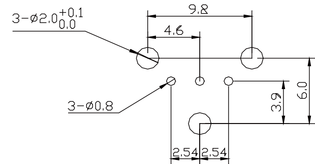
PCB Layout for Electrical Circuit
