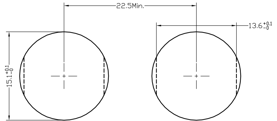
PANEL CUT-OUT
