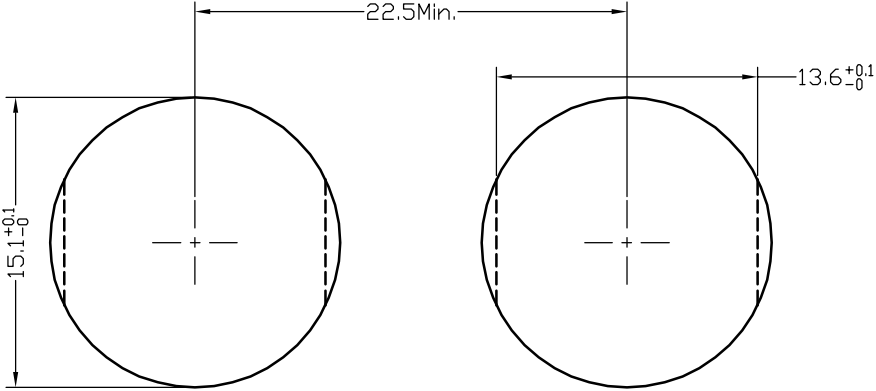
PANEL CUT-OUT
