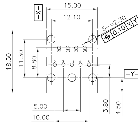
RECOMMENDED PCB LAYOUT COMPONENT SIDE TOLERANCE: \pm 0.05
