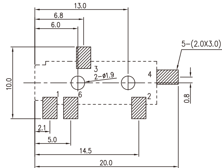
T:1.6 Dimensions of PC board holes Tolerance : \pm 0.05 (Printed-top view)
