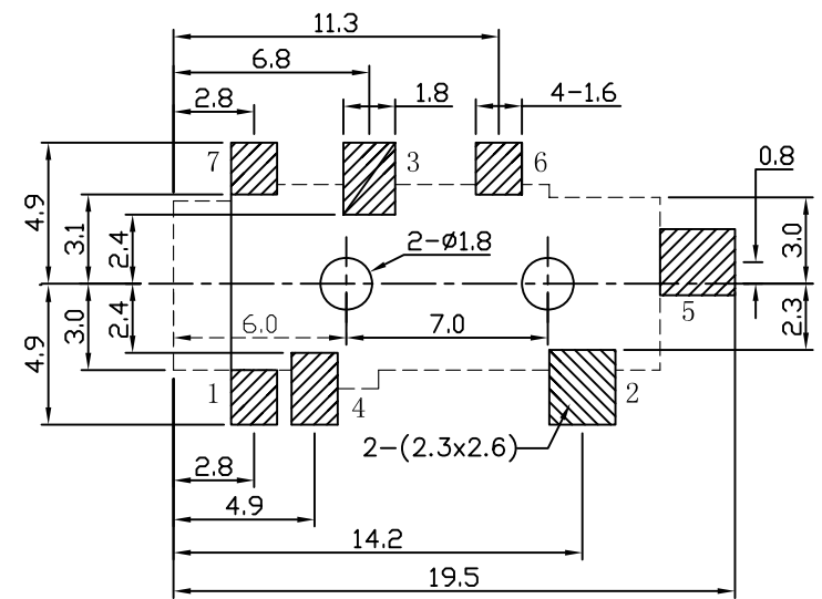
T:1.6 Dimensions of PC board holes Tolerance : ±0.05(Printed-top view)
