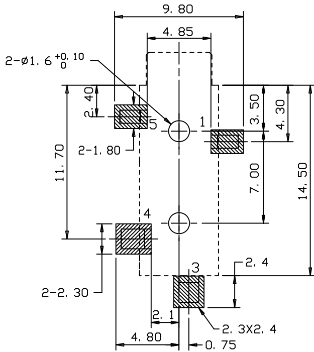
Recommended PADS Layout Tolerance ±0.2mm <TOP VIEW>
