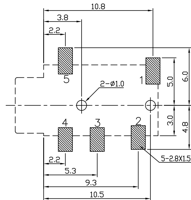
T:1.6 Dimensions of PC board holes Tolerance : \pm 0.05 (Printed-top view)
