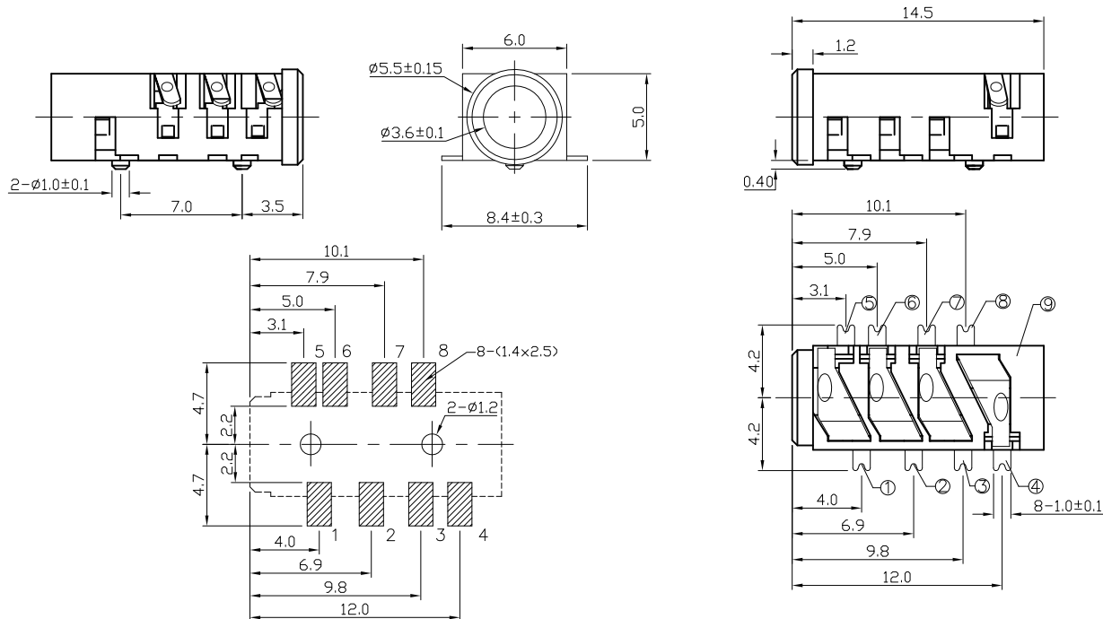
T:1.6 Dimensions of PC board holes Tolerance : \pm 0.1 (Printed-top view)
