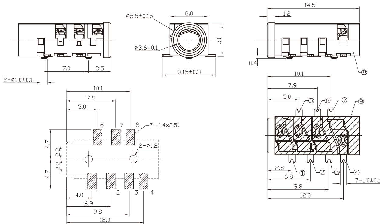
T:1.6 Dimensions of PC board holes Tolerance : ±0.05(Printed-top view)
