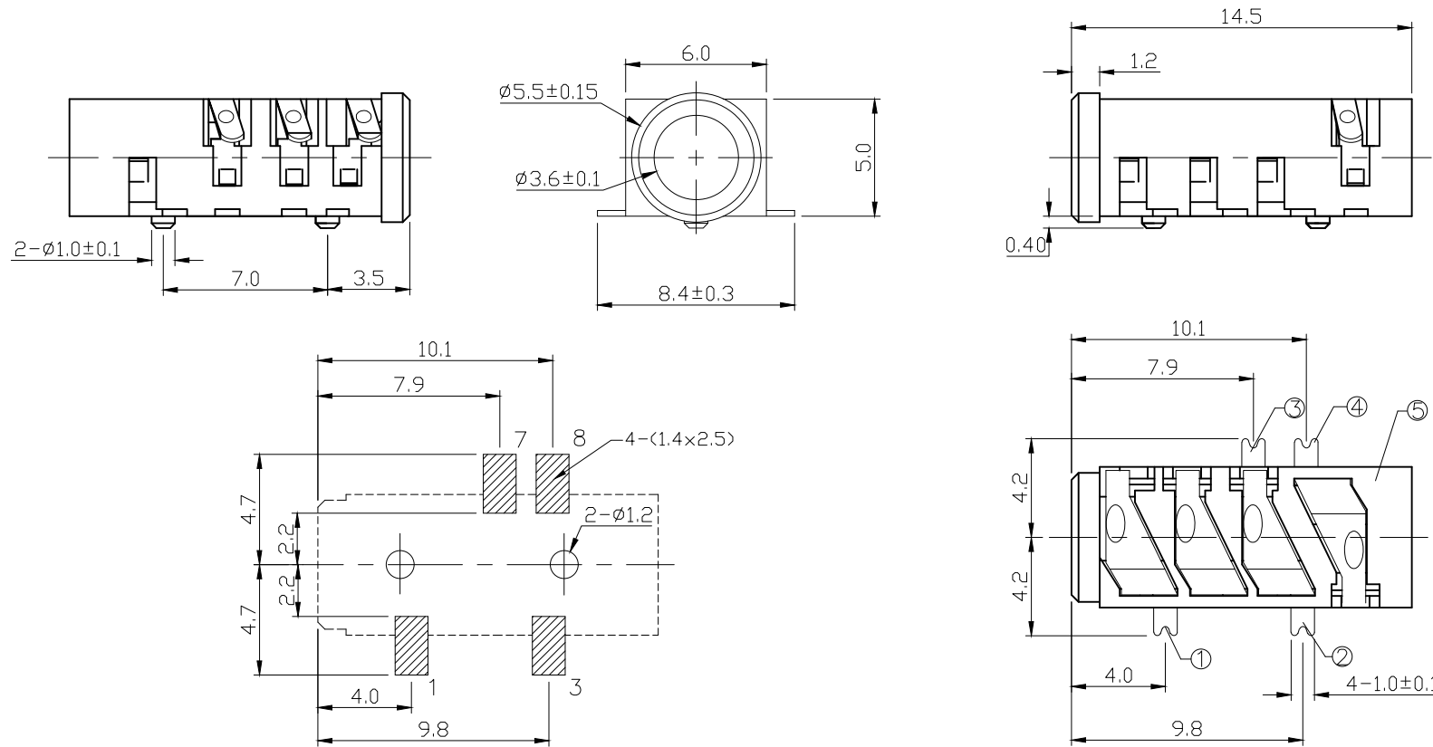
T:1.6 Dimensions of PC board holes Tolerance : \pm 0.05 (Printed-top view)
