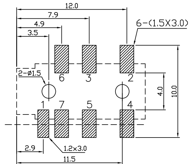
T:1.6 Dimensions of PC board holes
