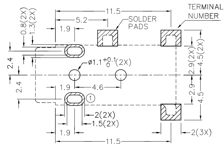
RECOMMENDED PCB LAYOUT TOLERANCE: \pm 0.05 (TOP VIEW)
