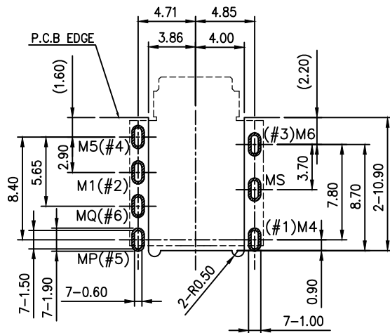
RECOMMENDED PADS LAYOUT <TOP VIEW>
