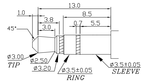
PLUG (SCALE 10:1)
