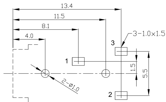
P.C.B. LAYOUT(±0.1) (BOTTOM VIEW)
